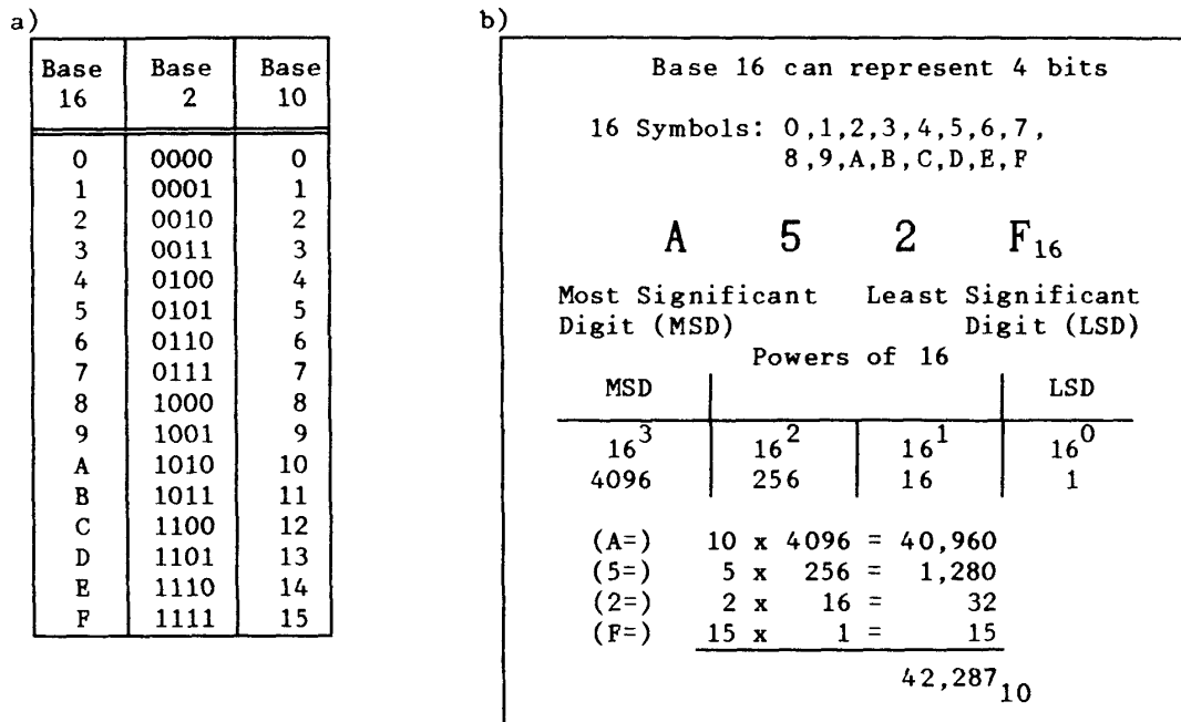
Figure 5 Hexadecimal Numbers
